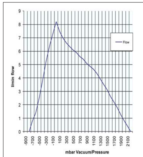
Gas Flow Curve
