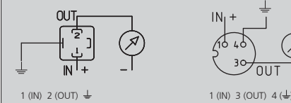
1 (IN) 2 (OUT) 1 (IN) 3 (OUT) 4 (GND)
